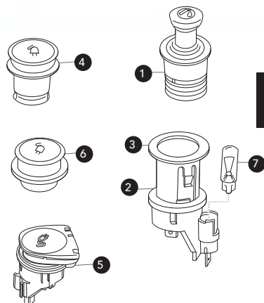
Cigar Lighter Switch
