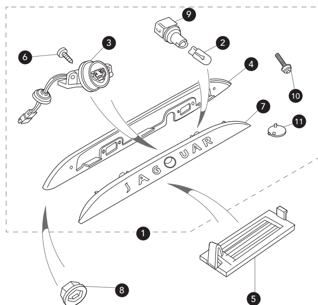
Numberplate Lamp Assembly
